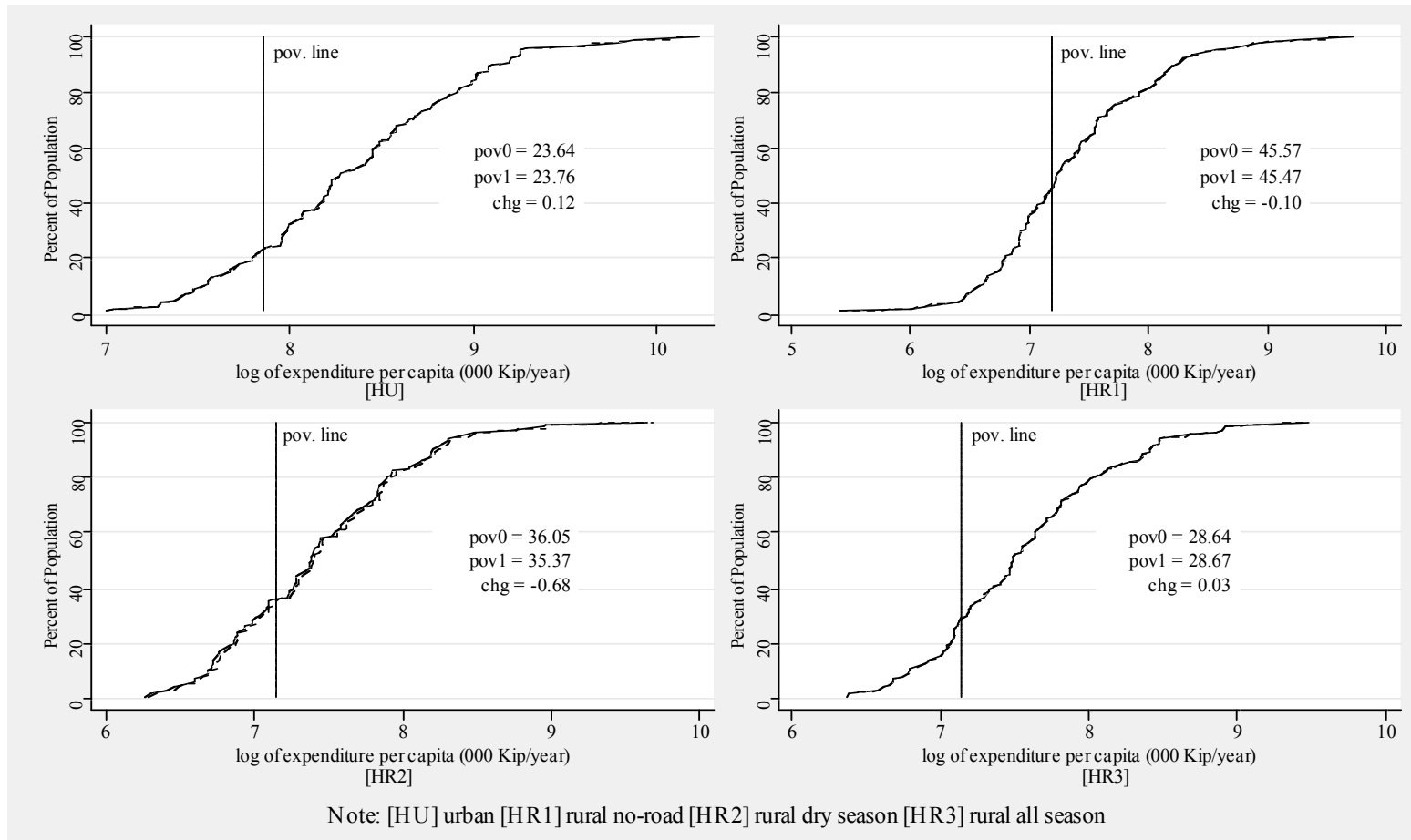
Figure 4.1 Changes in the cumulative distribution of real expenditures in Simulation S1
