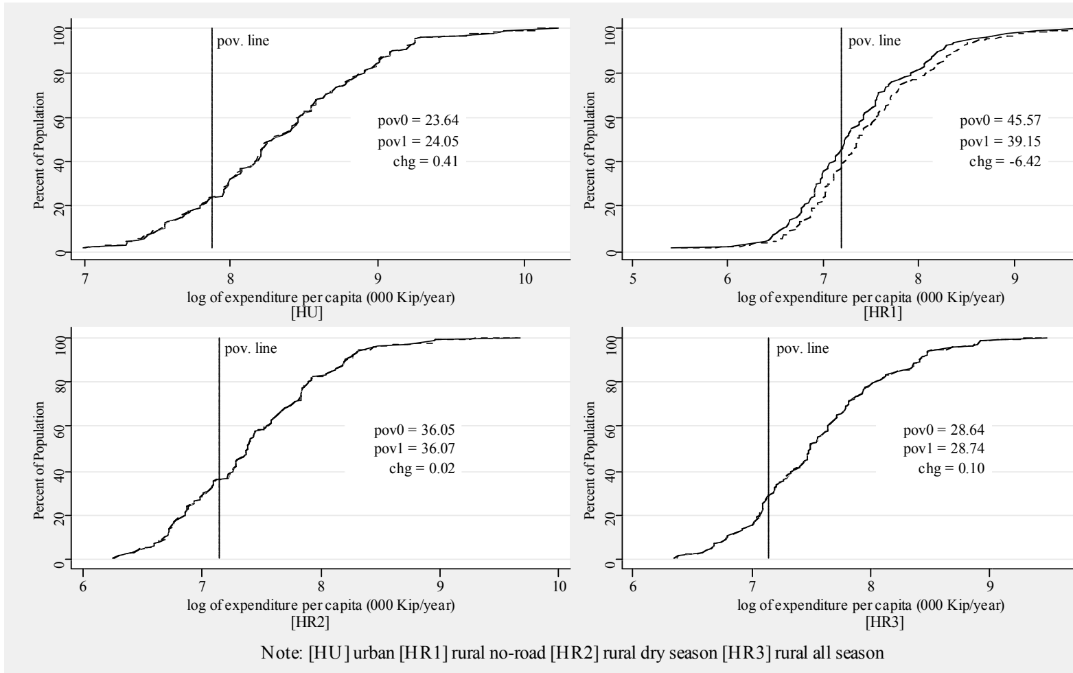
Figure 4.2 Changes in the cumulative distribution of real expenditures in Simulation S2
