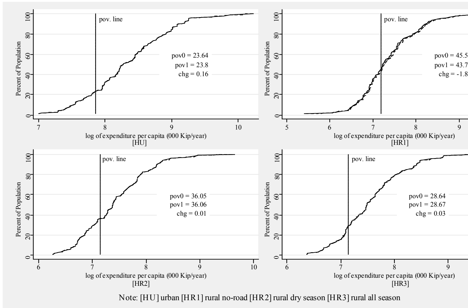
Figure 4.4 Changes in the cumulative distribution of real expenditures in Simulation S4
