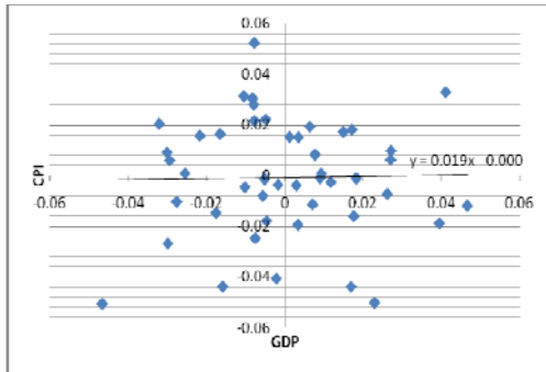
Figure 2: Indonesia's AS and AD Curves, 1994q3-2005q4
